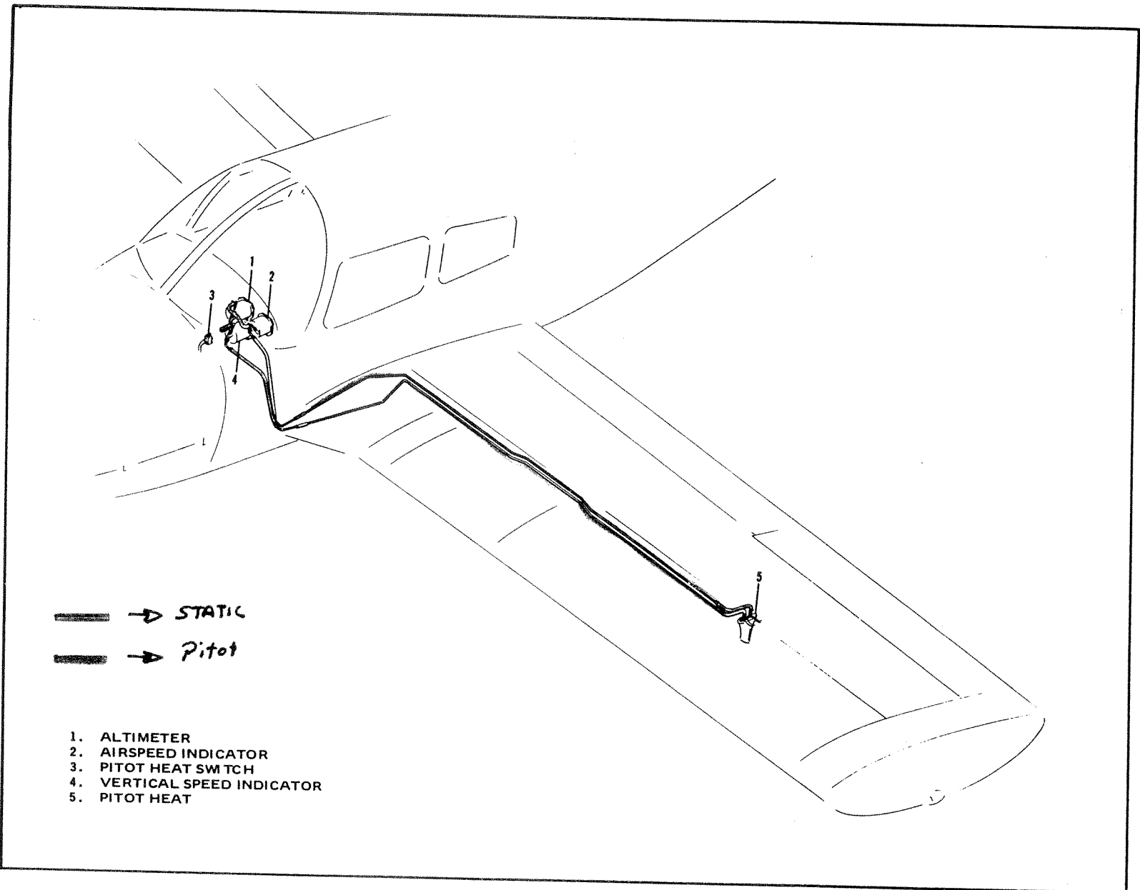
Pitot-Static System
